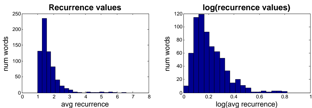
Figure 5-4: Histogram of raw and log-transformed recurrence values. This is for the set of words the child learned.
