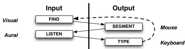
Figure 3-2: The FIND-SEGMENT-LISTEN-TYPE functional decomposition of traditional manual transcription approaches. Repeatedly switching between different input modalities and output devices is inefficient, but automating some of these tasks can speed up the transcription process.
