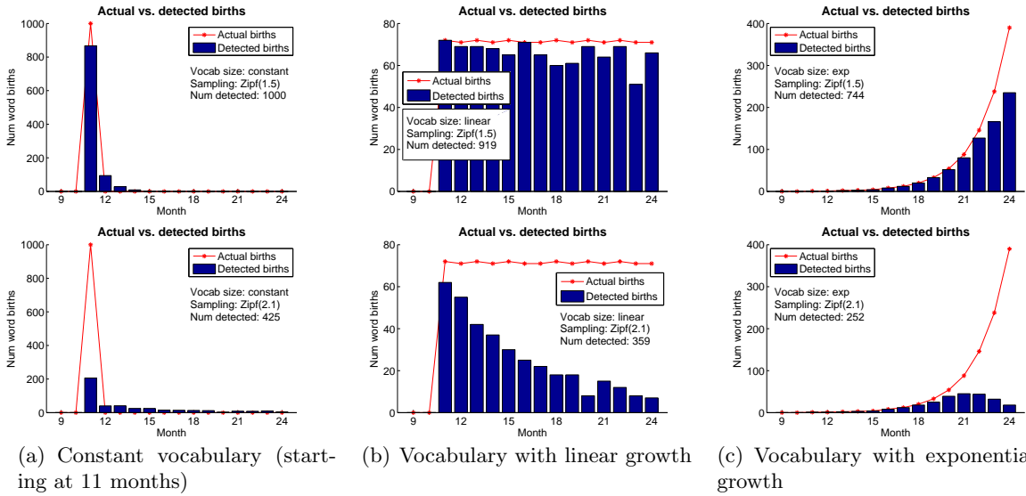
Figure 4-10: Actual and detected word births for constant, linear and exponential vocabularies. Words are uttered at random according to a Zipfian distribution with parameter \alpha = 1.5 (top row) or \alpha = 2.1 (bottom row). A fixed k = 5000 tokens are uttered per day, and in all cases the true vocabulary is 1000 words by 24 months. The only model in which true vocabulary continues to grow while the observed vocabulary has a “shark fin” shape is the exponential + Zipf(2.1) combination (bottom right, detail in figure 4-11).
