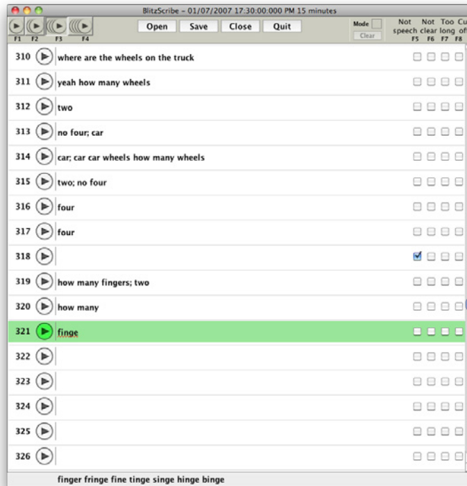
(a) BlitzScribe user interface
