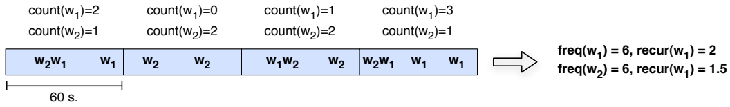
Figure 5-3: Illustration of the recurrence calculation for words w_1 and w_2 . Note that they could both have the same frequency and different recurrence values, as w_1 only occurs in three intervals while w_2 occurs in four intervals. In practice, the number of intervals generally differs for each word, since the rightmost interval depends on the AoA for the word under consideration.
